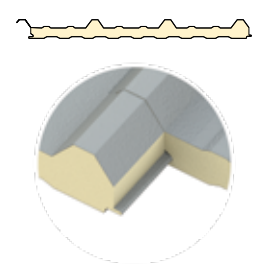
LS-36™ INSULATED METAL ROOF & WALL EXPOSED FASTENERS
