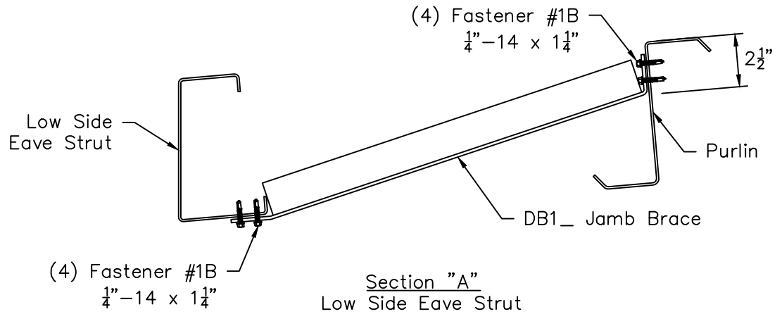
Jamb Brace at Eave Strut to Purlin
