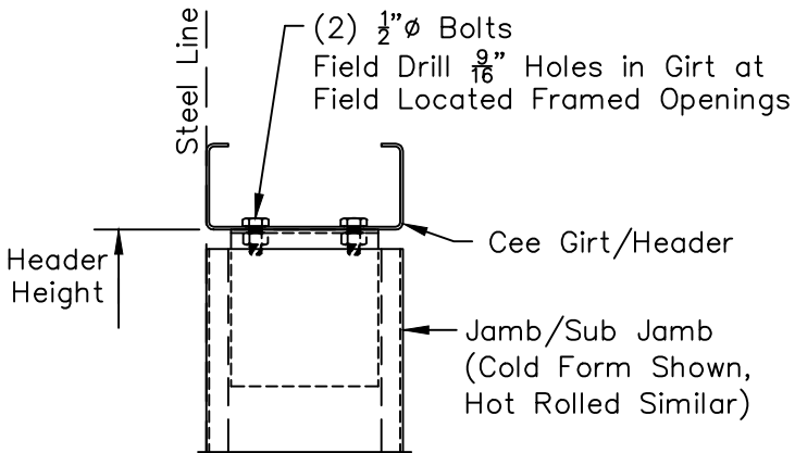
Jamb/Sub Jamb to Cee Girt/Header
