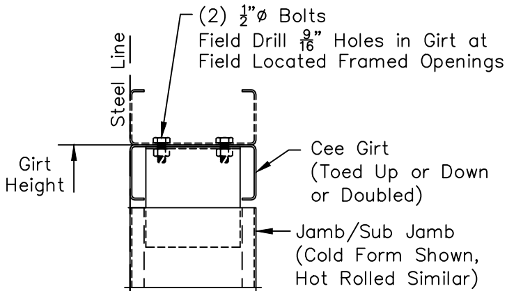
Jamb/Sub Jamb to Cee Girt
