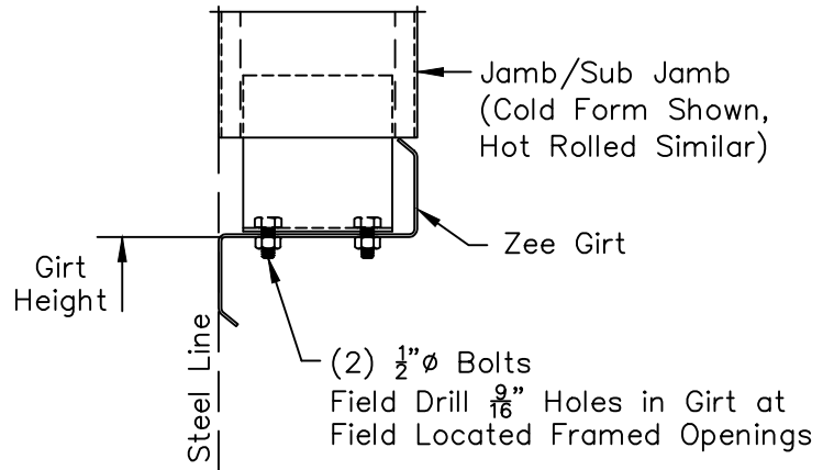
Jamb/Sub Jamb to Zee Girt
