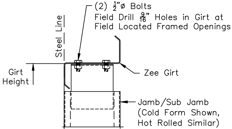
Jamb/Sub Jamb to Zee Girt
