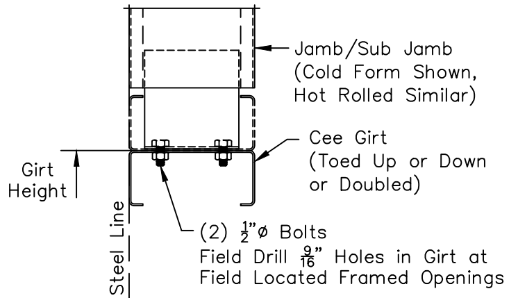
Jamb/Sub Jamb to Cee Girt
