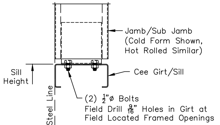
Jamb/Sub Jamb to Cee Girt/Sill
