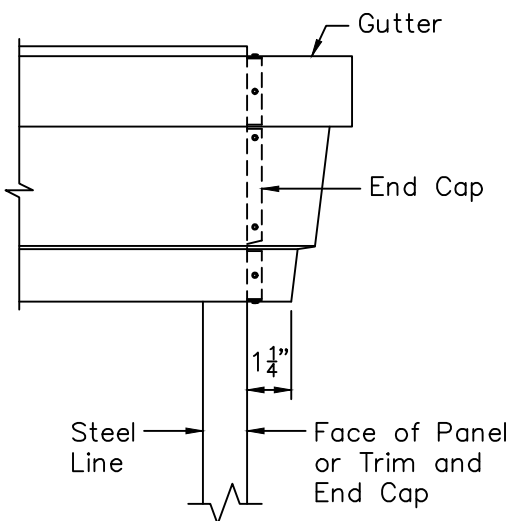
Gutter Placement
