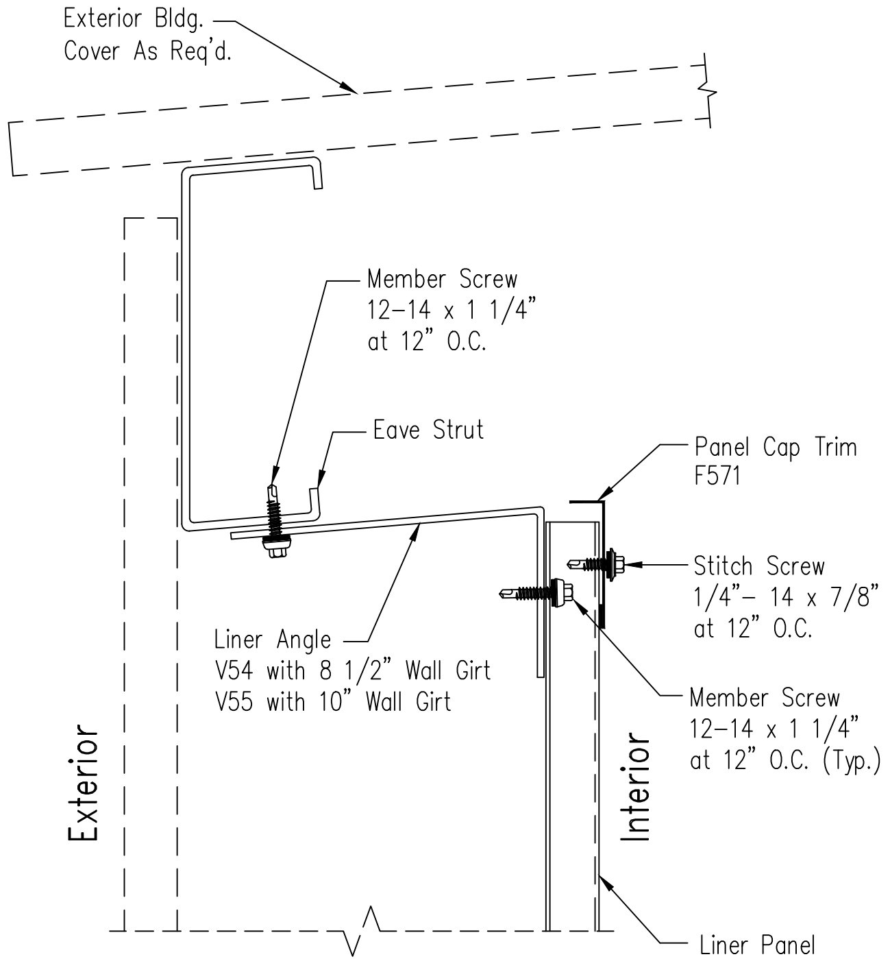
Section At Eave
