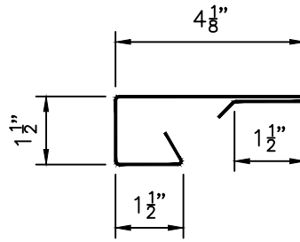
Jamb Trim F482 Top View
