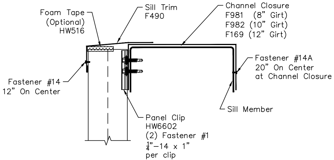
Section Thru Sill
