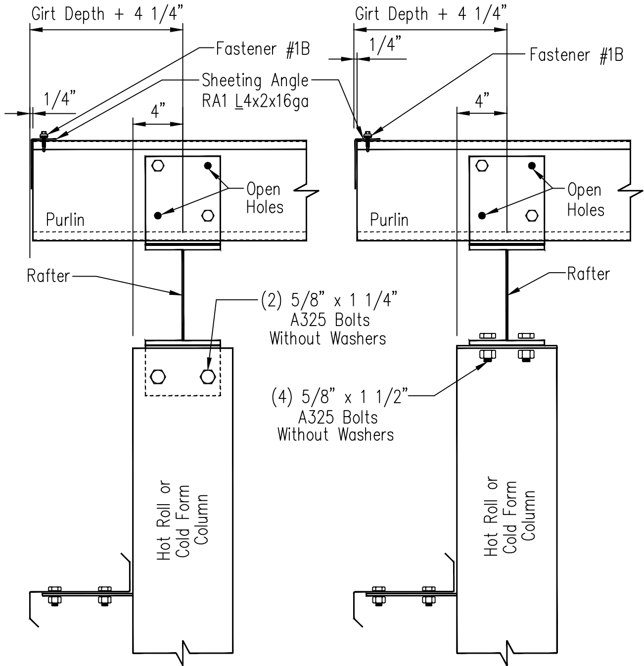
2 Bolt Connection
