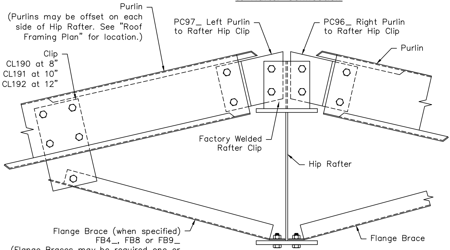
Top View of Purlin to Rafter Connection
