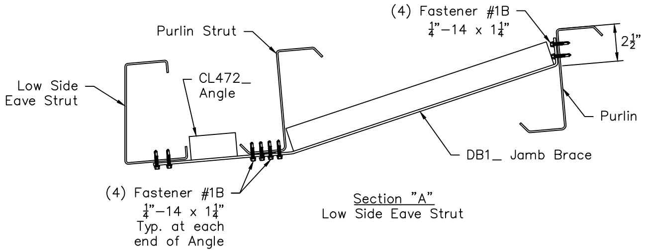
Jamb Brace at Eave Strut to Purlin
