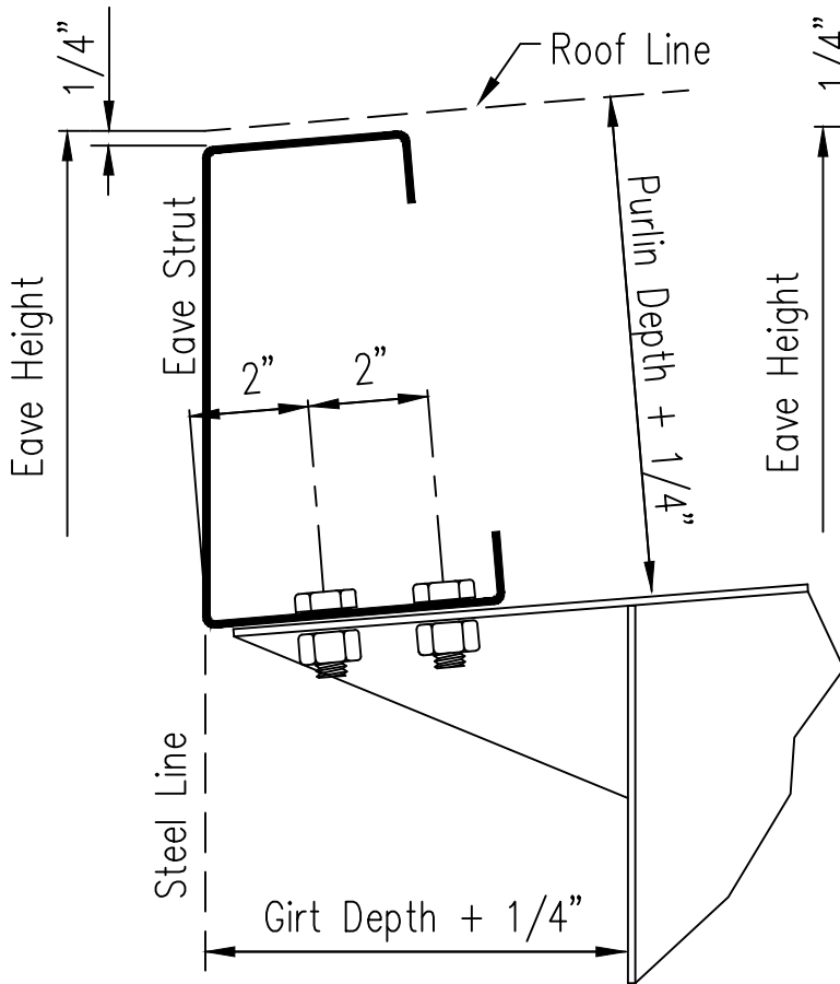
By-Pass Girts
