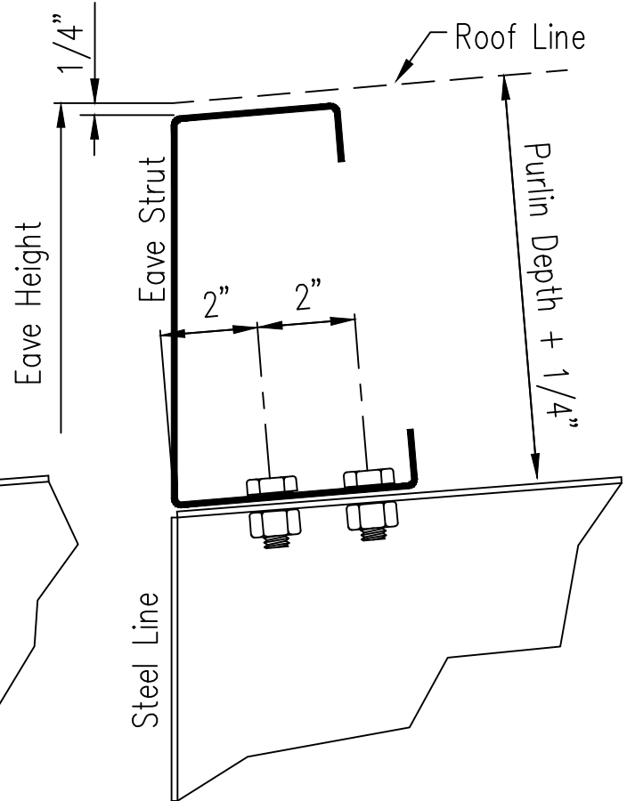
Flush Girts
